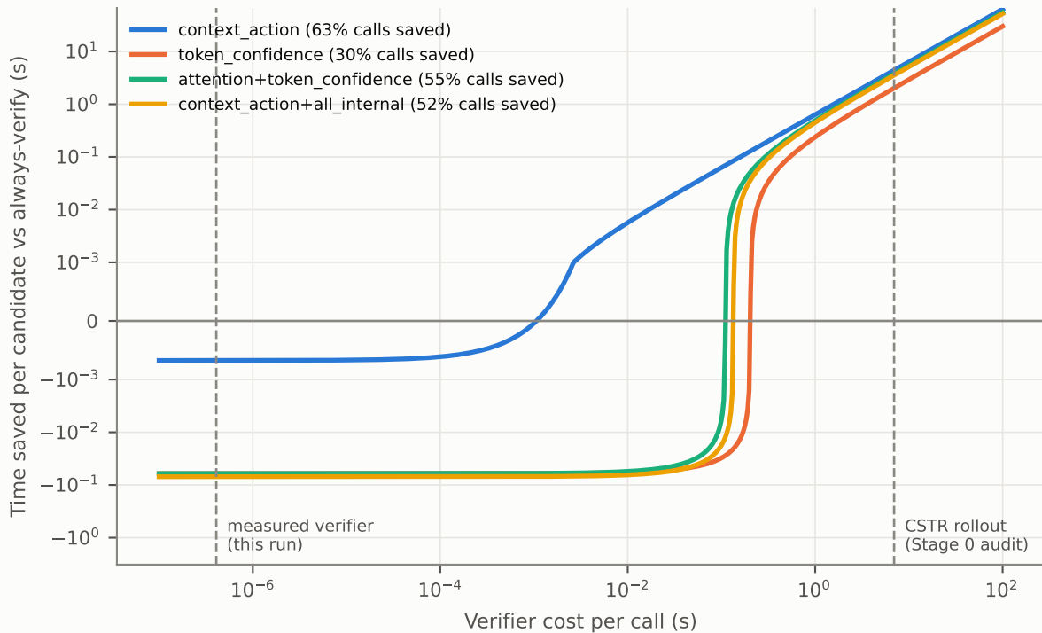
Time saved vs verifier cost (point, \alpha = 0.1 , \beta = 0.1 ; FSM routing and overhead)
