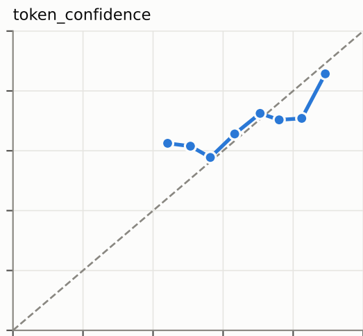
Reliability (dev_thr) (dashed: perfect calibration; bins with n < 5 hidden)
