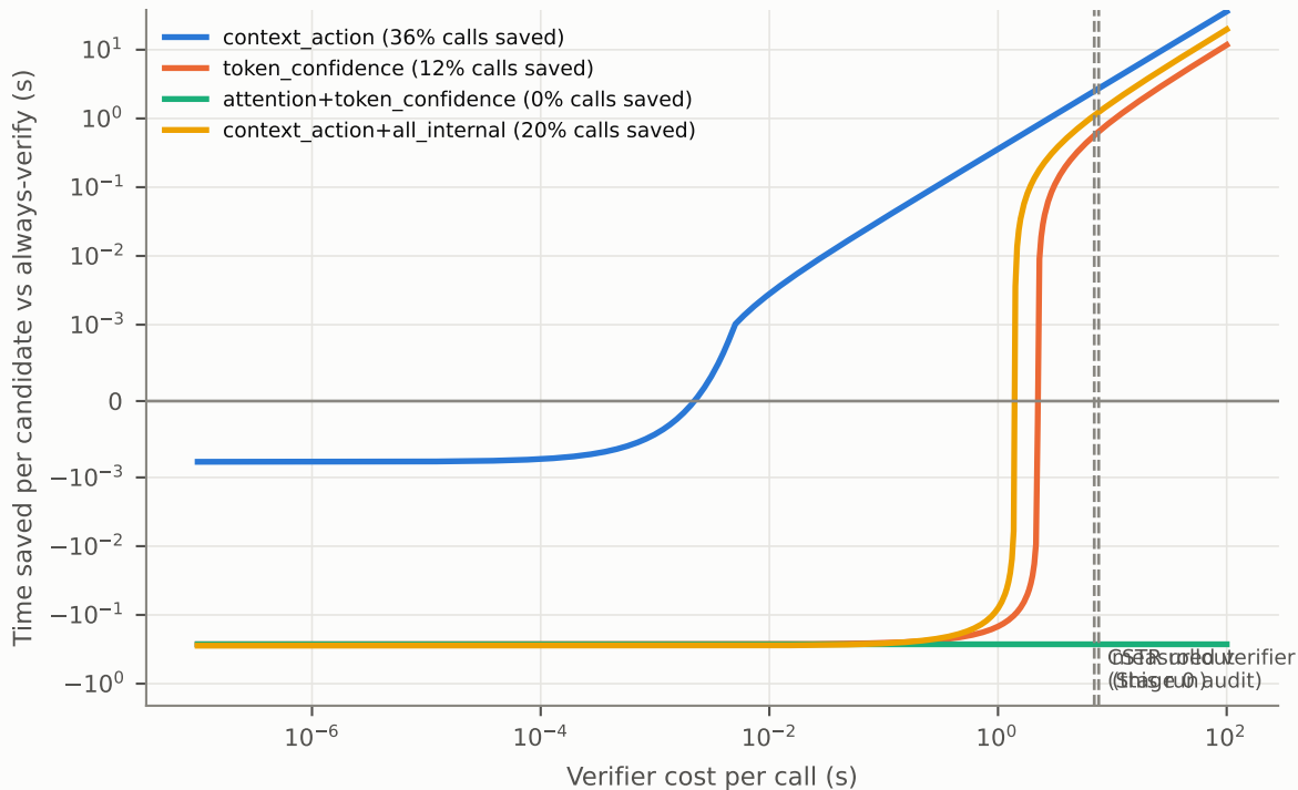
Time saved vs verifier cost (point, \alpha = 0.0 , \beta = 0.1 ; CSTR routing and overhead)
