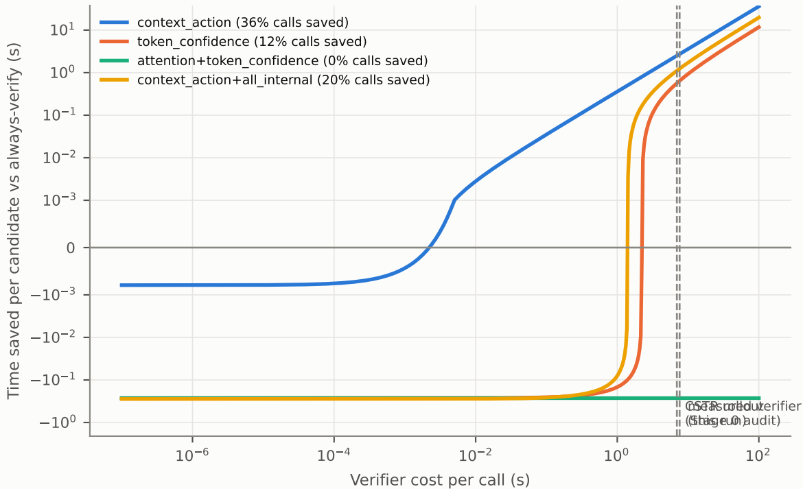
Time saved vs verifier cost (point, \alpha = 0.05 , \beta = 0.05 ; CSTR routing and overhead)
