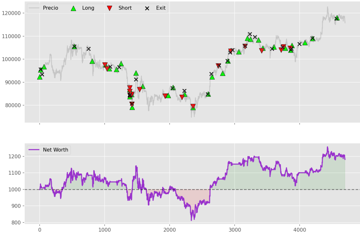
Operativa TRANSFORMER (Seed 1011) | Retorno: 18.12%
