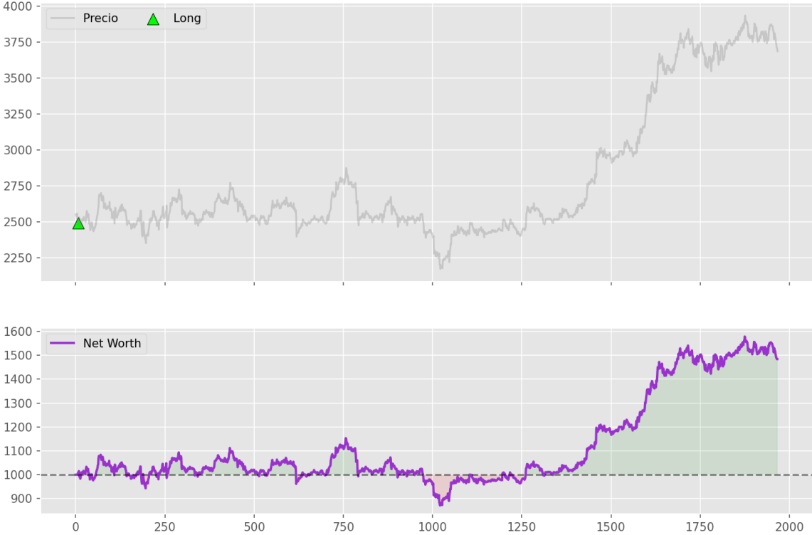
Operativa TRANSFORMER (Seed 456) | Retorno: 48.44%
