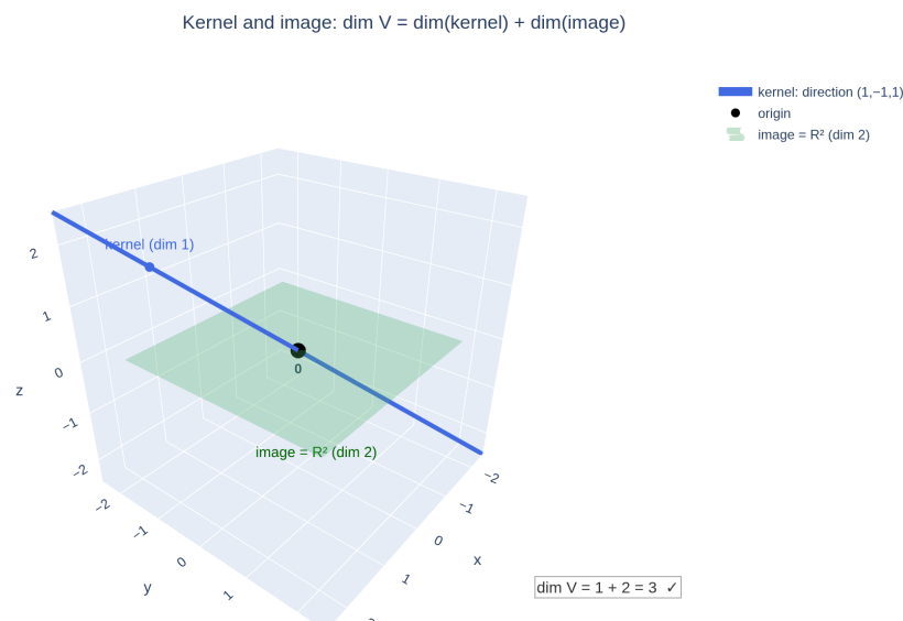
Figure 9: Kernel and image of a linear map: what collapses (the kernel, here a line) and what survives; \dim V = \dim(\text{kernel}) + \dim(\text{image}) .
