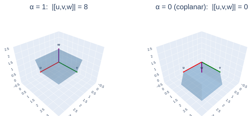
Figure 19: Coplanarity \iff volume 0: as the third vector approaches the plane of the other two, the parallelepiped flattens and [u, v, w] \rightarrow 0 .
