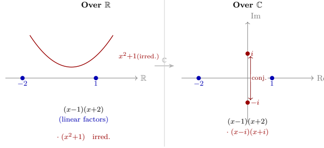
Figure 6: Over \mathbb{R} a polynomial factors into linear and irreducible quadratic factors; over \mathbb{C} those quadratics open up into pairs of conjugate roots.
