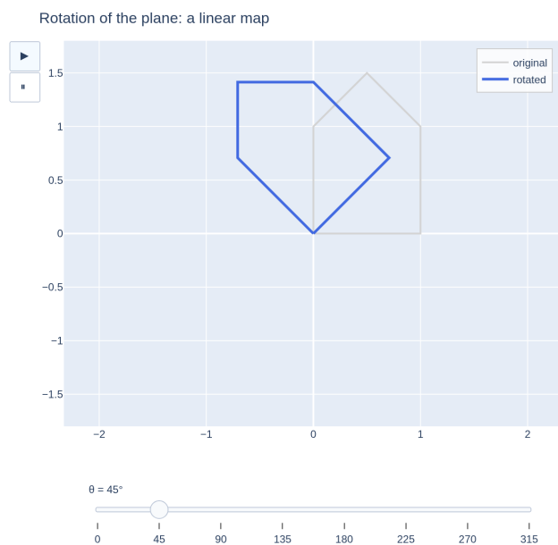
Figure 8: The rotation of the plane is a linear map: every vector is transformed by rotating it through the same angle (here, a figure and its rotated copy). [see interactive version]
