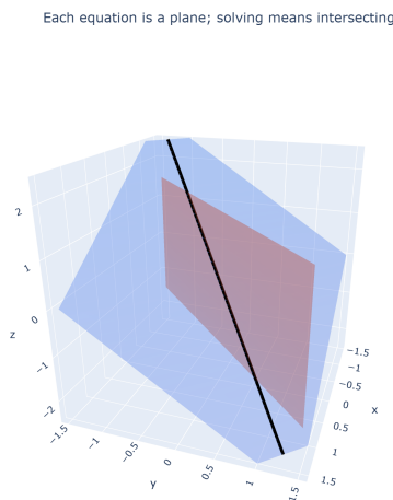
Figure 5: Each equation of a system is a plane in \mathbb{R}^3 ; the solution is their intersection (here, a line).
