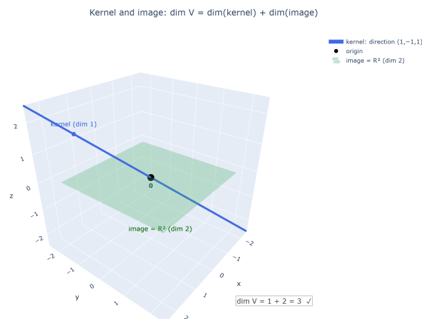
Figure 9: Kernel and image of a linear map: what collapses (the kernel, here a line) and what survives; \dim V = \dim(\text{kernel}) + \dim(\text{image}) .
