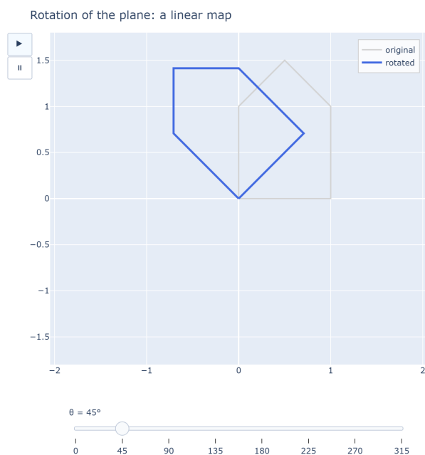
Figure 7: The rotation of the plane is a linear map: every vector is transformed by rotating it through the same angle (here, a figure and its rotated copy). [see interactive version]
