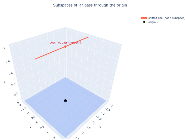
Figure 4: A subspace of \mathbb{R}^3 passes through the origin (a plane, here); a shifted line that misses 0 is not a subspace.
