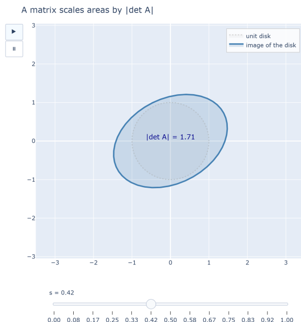
Figure 8: A 2 \times 2 matrix transforms the unit disk into an ellipse, multiplying the area by |\det A| .
