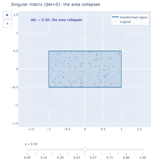
Figure 12: As \det A \rightarrow 0 the transformation flattens the area to zero: a singular matrix collapses space to a lower dimension.
