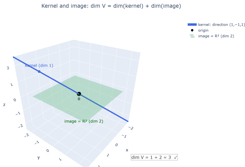
Figure 9: Kernel and image of a linear map: what collapses (the kernel, here a line) and what survives; \dim V = \dim(\text{kernel}) + \dim(\text{image}) .
