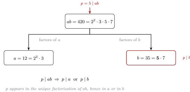
Figure 3: Via unique factorization, the primes of ab are those of a together with those of b ; if p \mid ab , p is one of them, hence it is “in” a or “in” b . For a composite like 6, its two primes can split between the factors.
