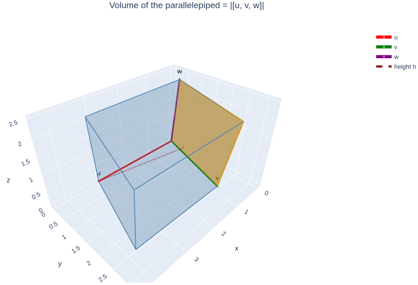
Figure 20: Parallelepiped with edges u, v, w from a common vertex: base the parallelogram of v, w (area \|v \times w\| ) and height \|\text{proj}_n u\| with n = v \times w ; if coplanar, it flattens onto a plane (volume 0).
