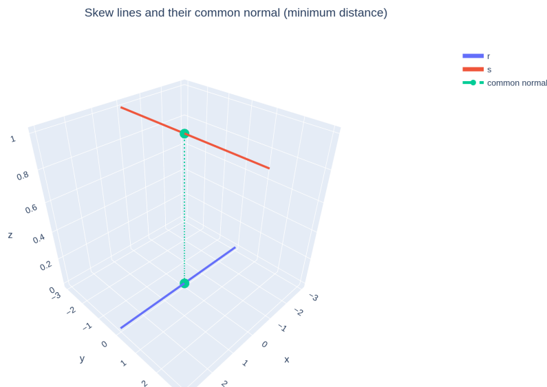
Figure 23: Two skew lines r, s and the segment of the common normal realizing the minimum distance; rotating the view shows that they do not meet.
