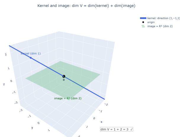
Figure 9: Kernel and image of a linear map: what collapses (the kernel, here a line) and what survives; \dim V = \dim(\text{kernel}) + \dim(\text{image}) . [see interactive version]
