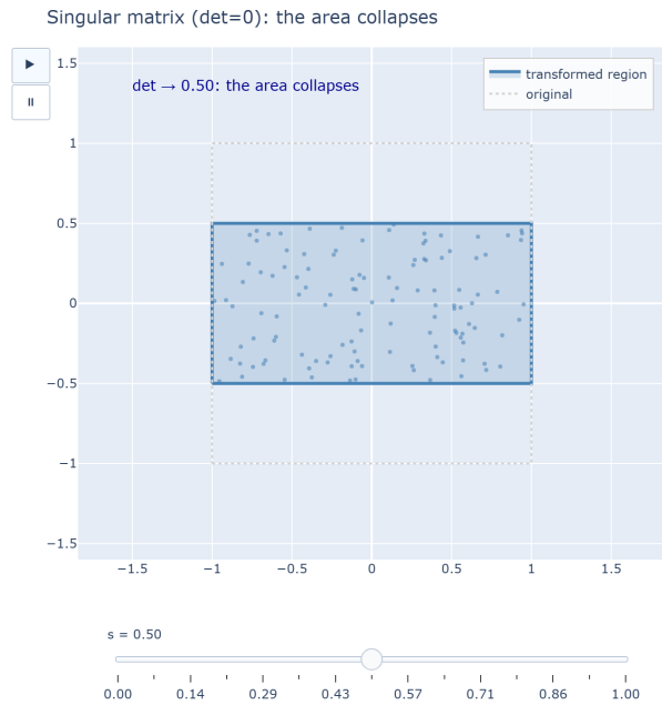
Figure 12: As \det A \rightarrow 0 the transformation flattens the area to zero: a singular matrix collapses space to a lower dimension. [see interactive version]
