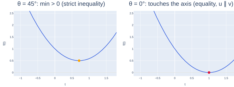
Figure 10: Cauchy–Schwarz, made visible: f(t) = \|u - tv\|^2 is a parabola that never dips below the axis; its discriminant being \leq 0 is the inequality, and it touches the axis (equality) only if u, v are proportional.
