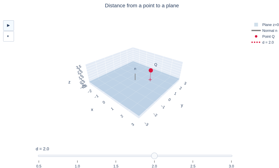
Figure 16: Distance from a point Q to a plane: the length of the perpendicular segment from Q to the plane (its projection onto the normal n ).
