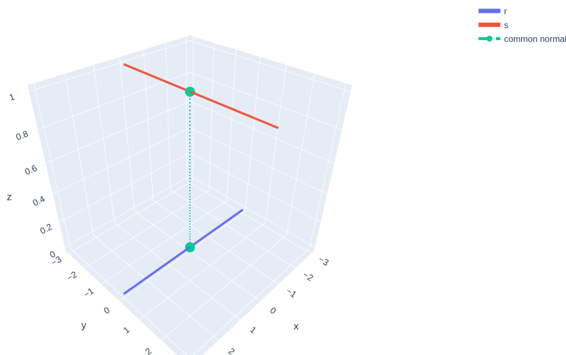
Figure 22: Two skew lines r, s and the segment of the common normal realizing the minimum distance; rotating the view shows that they do not meet.
