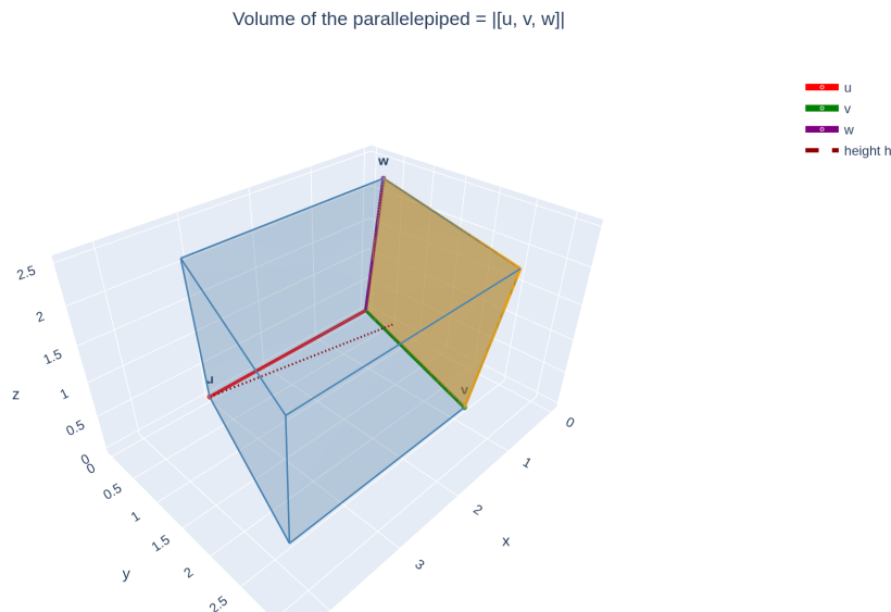
Figure 19: Parallelepiped with edges u, v, w from a common vertex: base the parallelogram of v, w (area \|v \times w\| ) and height \|\text{proj}_n u\| with n = v \times w ; if coplanar, it flattens onto a plane (volume 0).
