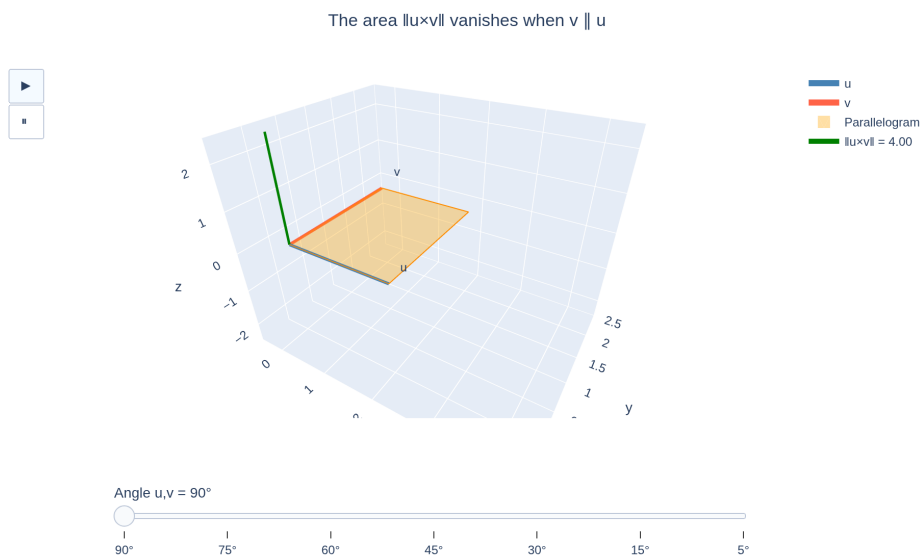
Figure 18: The area \|u \times v\| vanishes as v becomes parallel to u : the parallelogram flattens and u \times v \rightarrow 0 .
