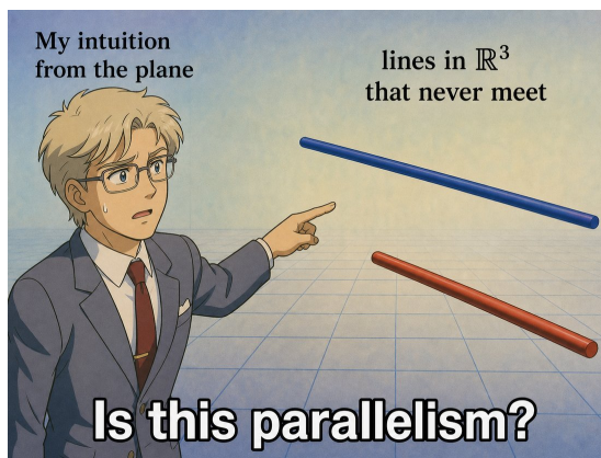
Figure 8: The plane reflex that space dismantles: in \mathbb{R}^2 , “they do not meet” forces “parallel”; in \mathbb{R}^3 the new case appears — skew lines — and the character’s question is exactly the mistake. The existence of skew lines is a dimensional phenomenon (see the note after Proposition 5.2.5).
