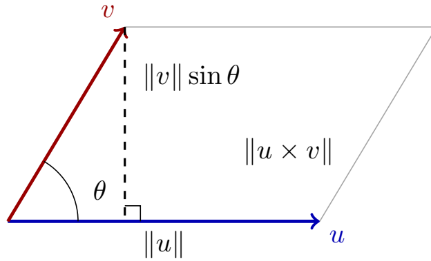
Figure 17: Parallelogram with sides u, v : base \|u\| and height \|v\| \sin \theta (the component of v perpendicular to u ); its area is \|u \times v\| .
