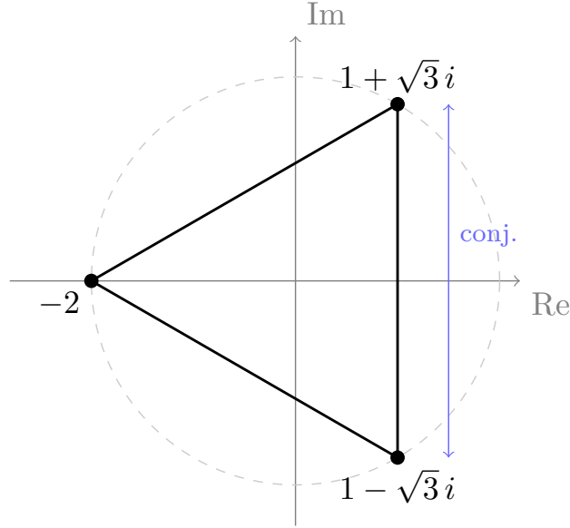
Figure 10: Solutions of z^3 = -8 : an equilateral triangle of radius 2 with one vertex at -2 and the others at 1 \pm \sqrt{3}i , symmetric with respect to the real axis ( z_2 = \bar{z}_0 ).
