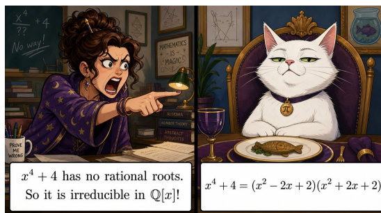
Figure 5: The classic mistake, so it is never forgotten: “no rational roots \Rightarrow irreducible” only holds in degrees 2 and 3 — from degree 4 on, a polynomial can factor into quadratics without having any root at all.
