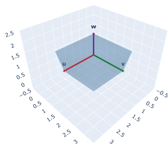
Figure 19: Coplanarity \iff volume 0: as the third vector approaches the plane of the other two, the parallelepiped flattens and |[u, v, w]| \rightarrow 0 .
