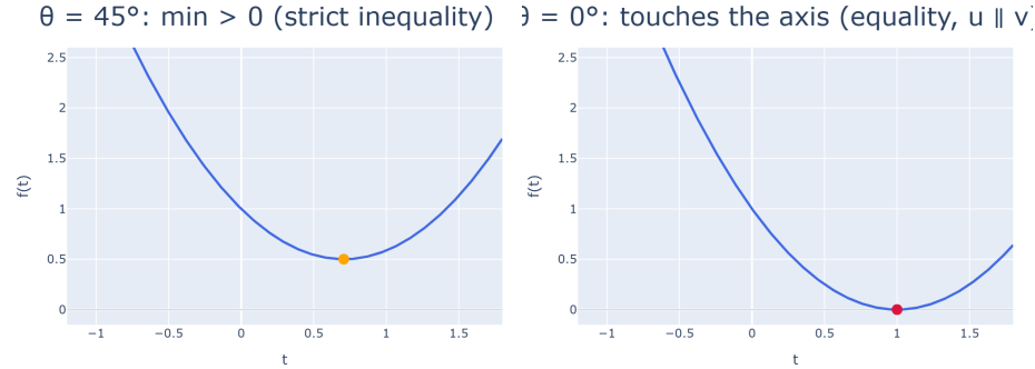
Figure 9: Cauchy–Schwarz, made visible: f(t) = \|u - tv\|^2 is a parabola that never dips below the axis; its discriminant being \leq 0 is the inequality, and it touches the axis (equality) only if u, v are proportional.
