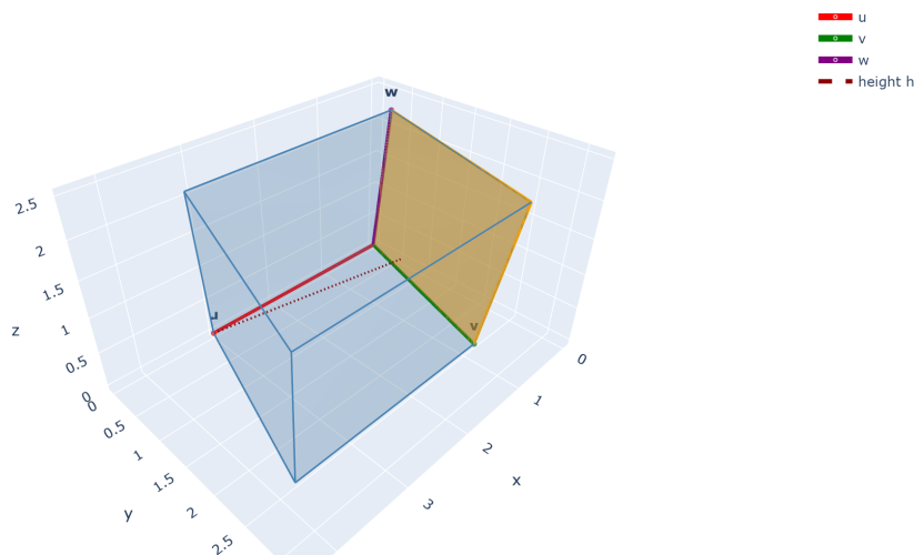
Figure 18: Parallelepiped with edges u, v, w from a common vertex: base the parallelogram of v, w (area \|v \times w\| ) and height \|\text{proj}_n u\| with n = v \times w ; if coplanar, it flattens onto a plane (volume 0).
