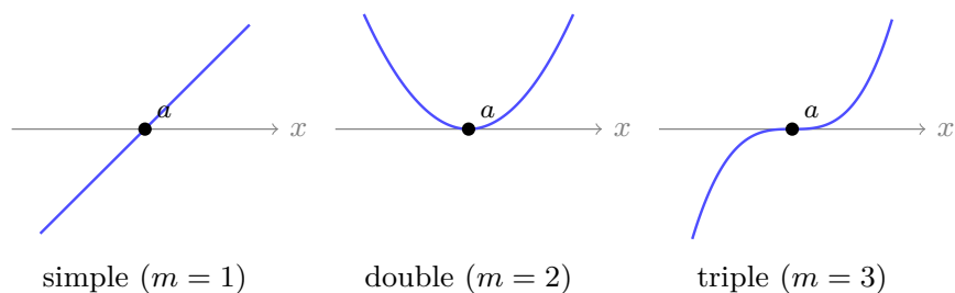
Figure 1: Three behaviours at the crossing x = a according to the multiplicity m : simple ( m = 1 ) crosses with nonzero slope; double ( m = 2 ) touches and bounces without changing sign; triple ( m = 3 ) crosses while flattening. Rule: odd m crosses, even m bounces.
