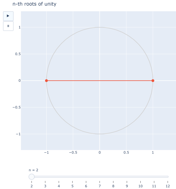
Figure 9: n -th roots of unity with a slider on n : as n varies, the number of vertices of the regular polygon inscribed in the unit circle changes. [see interactive version]
