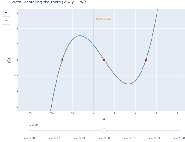
Figure 6: The substitution x = y - b/3 centers the roots at their mean (removes the quadratic term) — the first step of Cardano’s method. [see interactive version]
