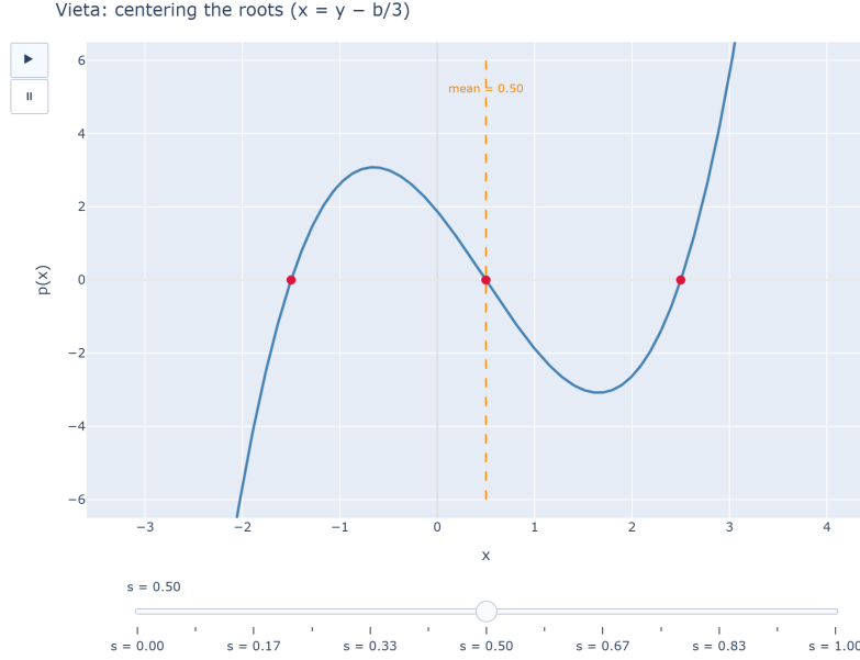
Figure 6: The substitution x = y - b/3 centers the roots at their mean (removes the quadratic term) — the first step of Cardano’s method.
