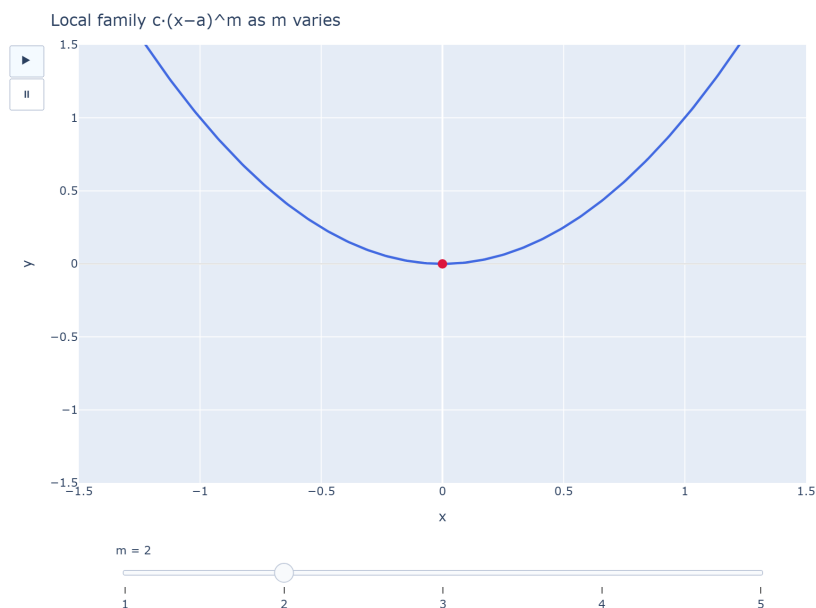
Figure 2: Local family c(x-a)^m as m = 1, 2, 3, \dots varies: the transition crossing (odd m ) \leftrightarrow bounce (even m ) and the increasing flattening of the contact. [see interactive version]
