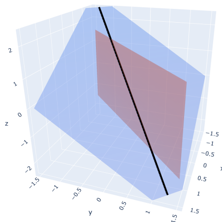
Figure 5: Each equation of a system is a plane in \mathbb{R}^3 ; the solution is their intersection (here, a line).
