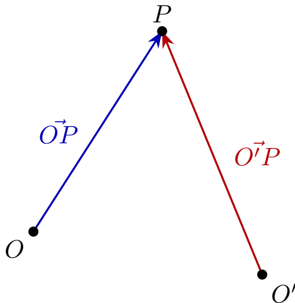
Figure 3: The base point is not intrinsic: the same P has different vectors \vec{OP} and \vec{O'P} depending on the origin, and hence different coordinates.
