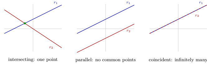
Figure 6: Relative positions of two lines in the plane (interactive version: drag the points of r_2 ): they meet at one point (intersecting), they do not meet (parallel) or they coincide.
