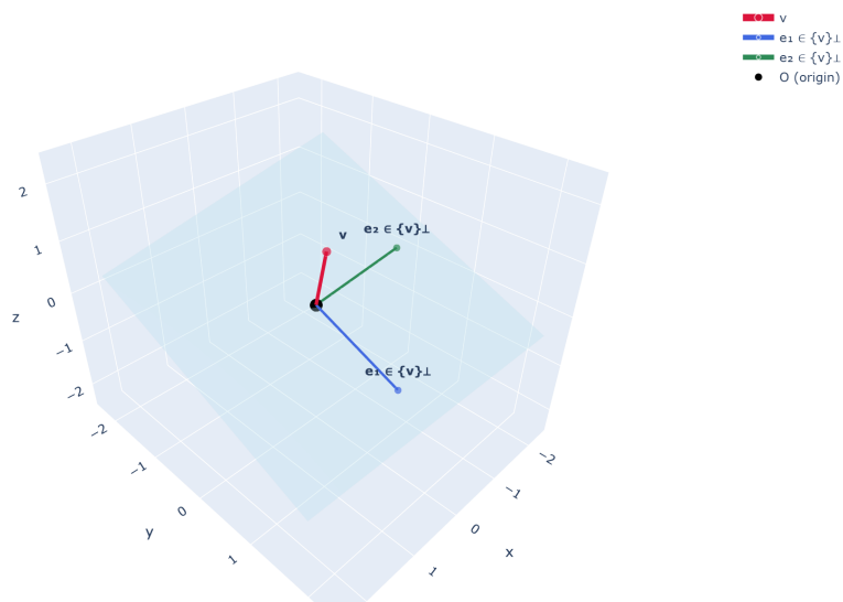
Figure 12: The orthogonal complement of a nonzero vector v is a plane through the origin: \{v\}^\perp = \{u : u \cdot v = 0\} . It is the basis of the idea of the “normal” of a plane.
