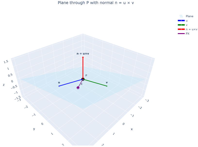
Figure 20: Plane through P with direction vectors u, v and the normal n = u \times v sticking out of the plane; a generic point X with \vec{PX} contained in the plane (perpendicular to n ).
