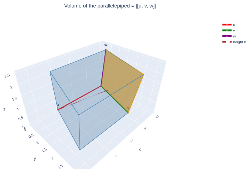
Figure 20: Parallelepiped with edges u, v, w from a common vertex: base the parallelogram of v, w (area \|v \times w\| ) and height \|\text{proj}_n u\| with n = v \times w ; if coplanar, it flattens onto a plane (volume 0).
