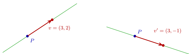
same point P : changing the direction vector reorients the whole line
