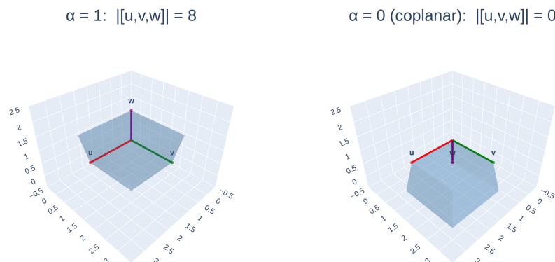
Figure 21: Coplanarity \iff volume 0: as the third vector approaches the plane of the other two, the parallelepiped flattens and |[u, v, w]| \rightarrow 0 .
