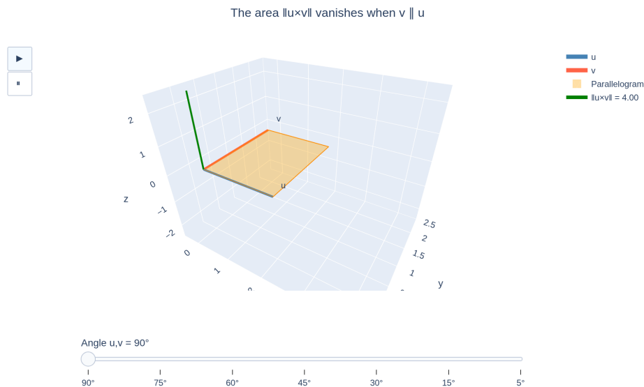
Figure 19: The area \|u \times v\| vanishes as v becomes parallel to u : the parallelogram flattens and u \times v \rightarrow 0 .
