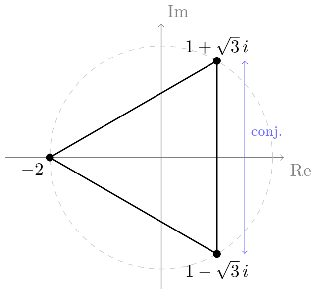
Figure 11: Solutions of z^3 = -8 : an equilateral triangle of radius 2 with one vertex at -2 and the others at 1 \pm \sqrt{3}i , symmetric with respect to the real axis ( z_2 = \bar{z}_0 ).
