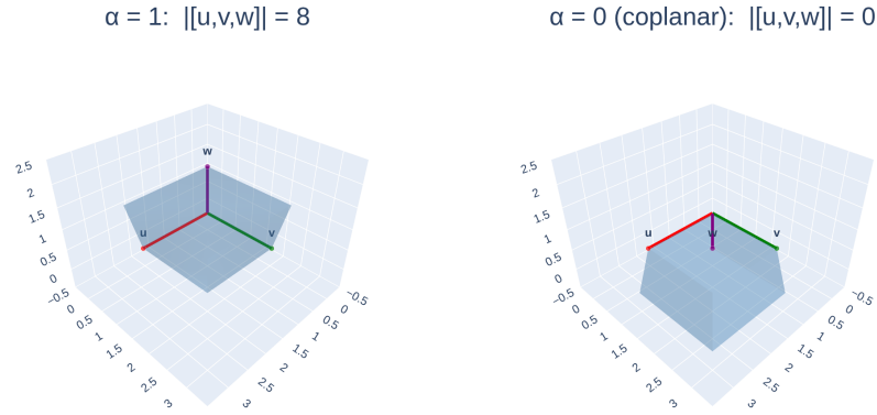
Figure 20: Coplanarity \iff volume 0: as the third vector approaches the plane of the other two, the parallelepiped flattens and |\llbracket u, v, w \rrbracket| \rightarrow 0 .
