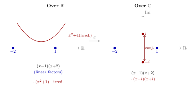
Figure 5: Over \mathbb{R} a polynomial factors into linear and irreducible quadratic factors; over \mathbb{C} those quadratics open up into pairs of conjugate roots.
