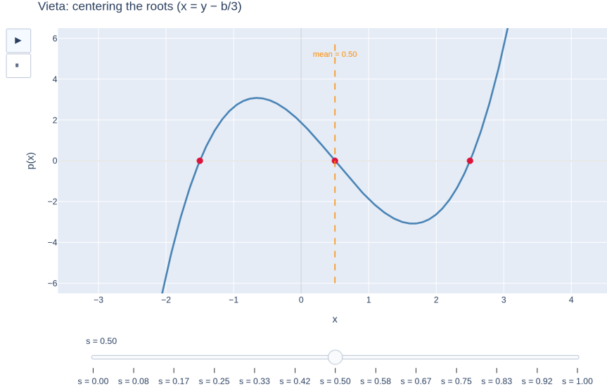
Figure 6: The substitution x = y - b/3 centers the roots at their mean (removes the quadratic term) — the first step of Cardano’s method.
