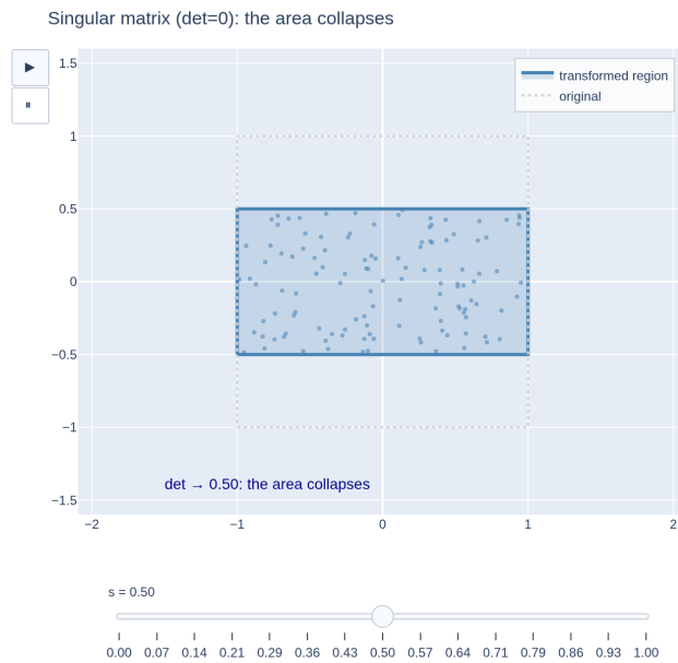
Figure 12: As \det A \rightarrow 0 the transformation flattens the area to zero: a singular matrix collapses space to a lower dimension.
