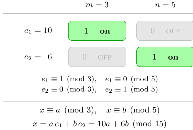
Figure 7: The CRT “switches”: e_1 is worth 1 modulo m and 0 modulo n , and e_2 the other way around; combining them, x = a e_1 + b e_2 solves the system.
