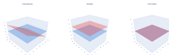
Figure 7: Relative positions of two planes in space: they meet in a line (intersecting), they are parallel or they coincide — with a slider running through the cases.
