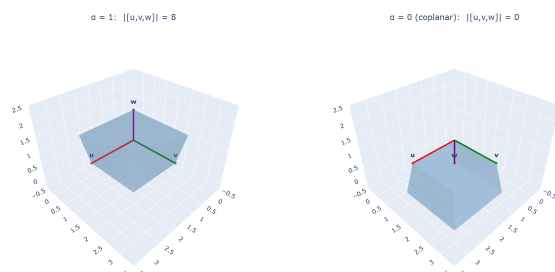
Figure 19: Coplanarity \iff volume 0: as the third vector approaches the plane of the other two, the parallelepiped flattens and |[u, v, w]| \rightarrow 0 .
