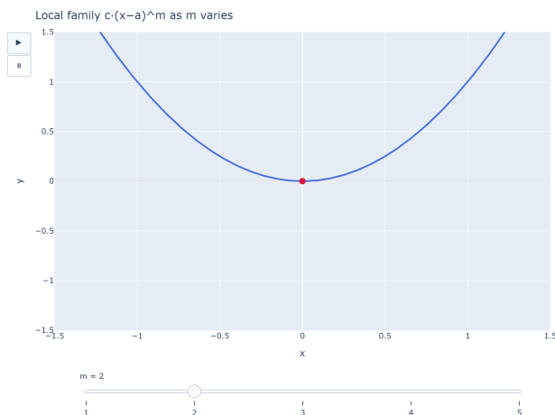
Figure 2: Local family c(x-a)^m as m = 1, 2, 3, \dots varies: the transition crossing (odd m ) \leftrightarrow bounce (even m ) and the increasing flattening of the contact.
