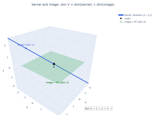
Figure 9: Kernel and image of a linear map: what collapses (the kernel, here a line) and what survives; \dim V = \dim(\text{kernel}) + \dim(\text{image}) .
