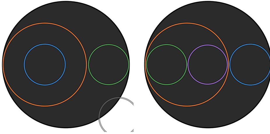
Figure 2: The n = 4 counterexample of Theorem 13: best fit (left) nests the 5 and loses the 4.8; the witness (right), realized by worst fit, places all four rings.
