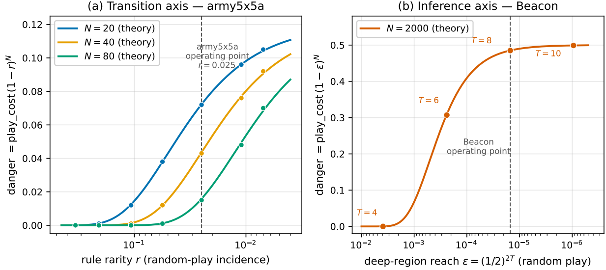
Figure 4: The danger law \text{danger} = \text{play\_cost} (1 - r)^N is a threshold in rarity, and the same law recurs on both halves of the CWM contract. Solid curves are the analytic law; markers are the measured operating points (Table 9 for panel (a), Table 15 for panel (b)). (a) Transition axis (army5x5a + material-at-cap), one curve per gate size N \in \{20, 40, 80\} : larger N pushes the threshold toward rarer rules. The deployed army5x5a instrument ( r = 0.0253 ) sits in the danger zone. (b) Inference axis (Beacon), fixed gate N = 2000 , swept over the deep-region reach \varepsilon = (1/2)^{2T} : harm climbs from \approx 0 at T = 4 to the full play cost by T \geq 8 . The x -axes are reversed (rarer to the right) so danger rises rightward in both panels.
