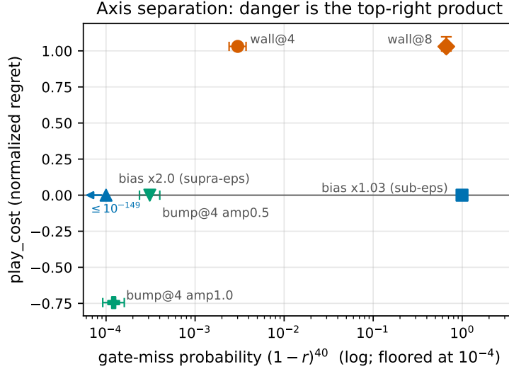
Figure 4: Table 4 as the danger quadrant: gate-miss probability (log) vs play_cost. Only the rare hard mode reaches the top right; danger is the product of the coordinates. Horizontal bars propagate each arm’s rarity interval through (1 - r)^{40} ; the play_cost axis carries a paired interval where per-episode returns exist and no bar where the arms are bit-identical, since there the difference is exactly zero rather than uncertain.
