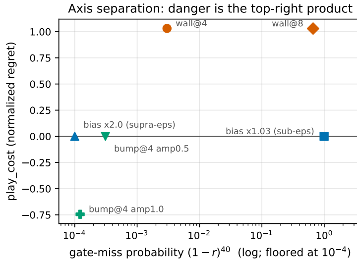
Figure 3: Table 5 as the danger quadrant: gate-miss probability (log) vs play_cost. Only the rare hard mode reaches the top right; danger is the product of the coordinates.
