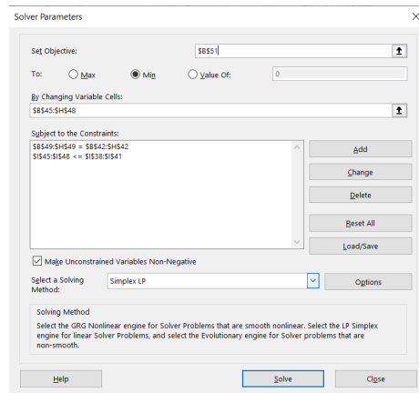
Figure 4: Excel Solver
