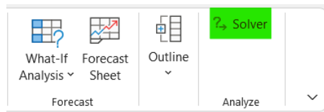
Figure 3: Solver Button
