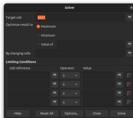
Figure 5: Calc Solver
