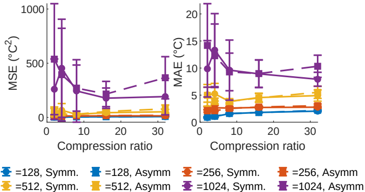
MSE and MAE vs ratio compression
