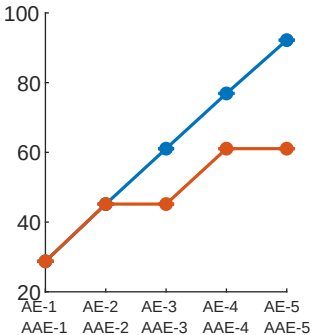
Encoder and decoder energy vs hidden layers
