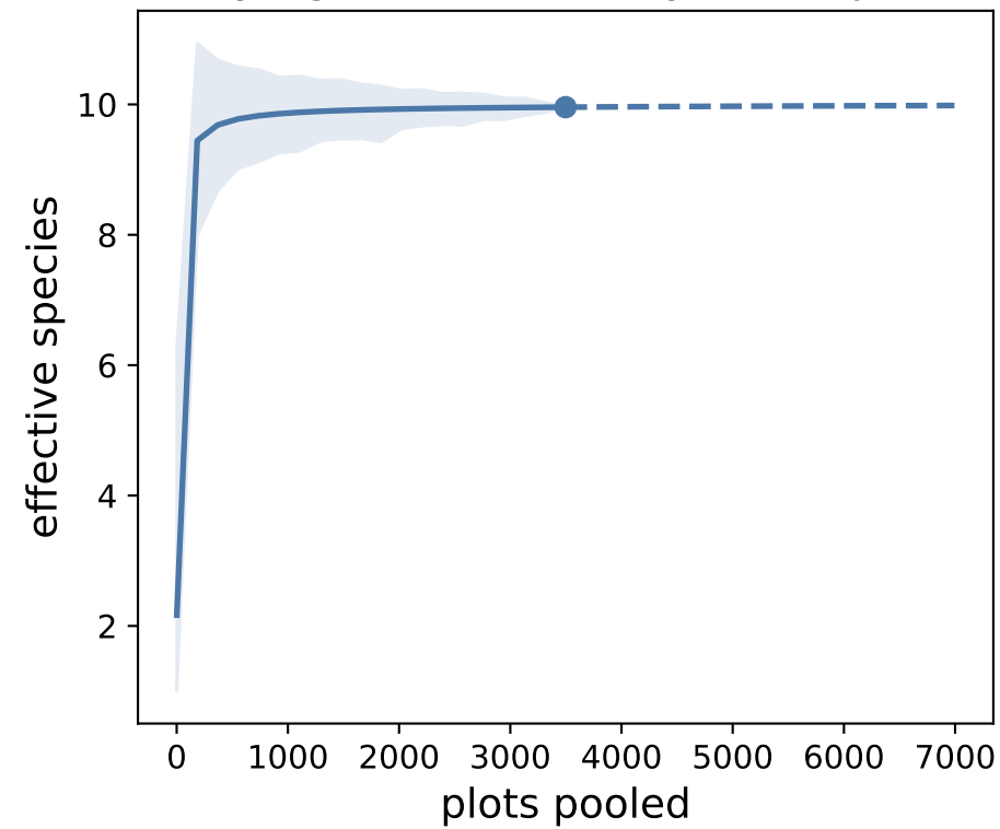
Phylogenetic diversity (PD), q = 1
