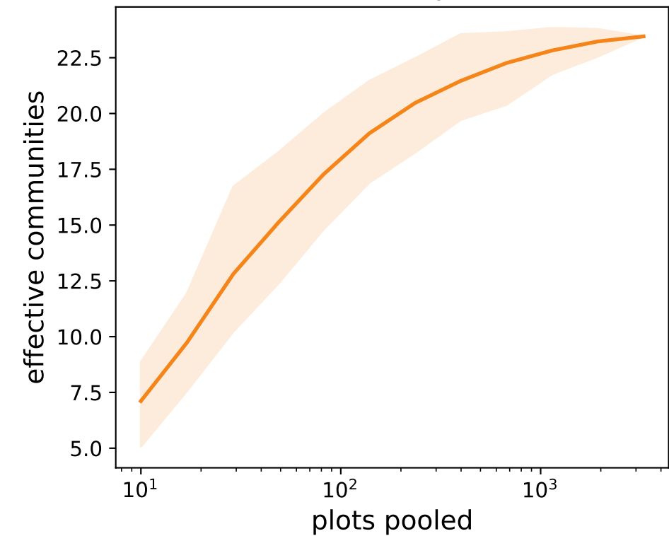
Hill beta, q = 1
