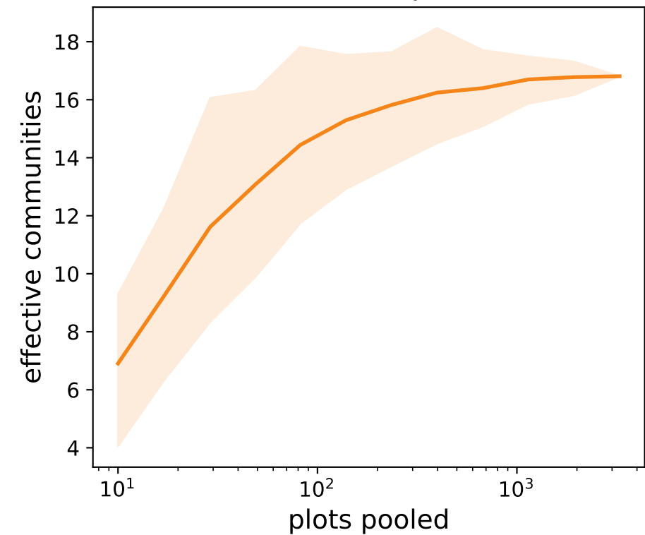
Hill beta, q = 2
