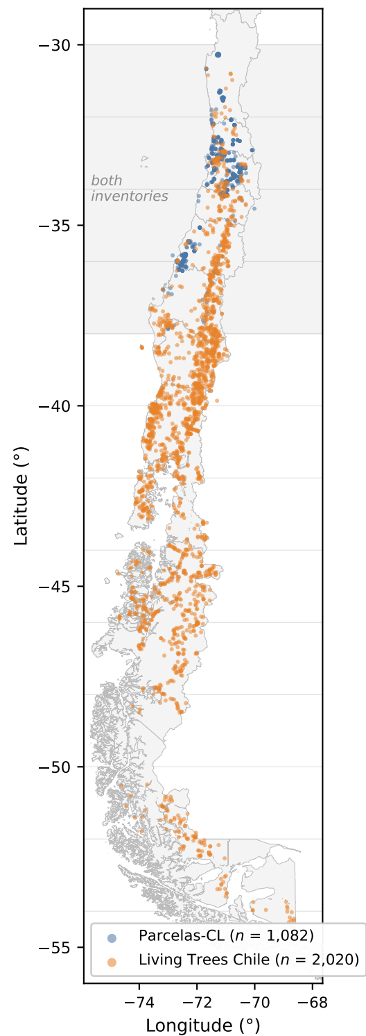
a Plot network
