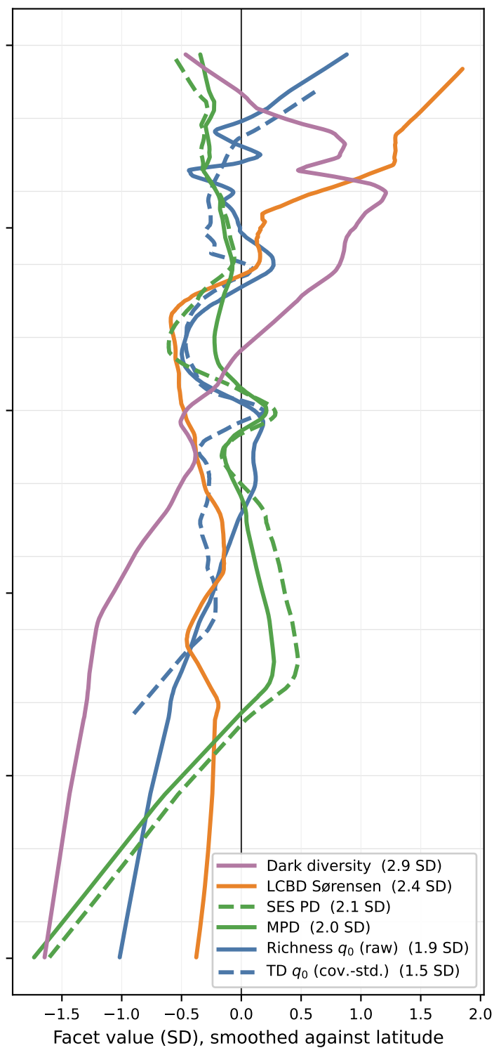
b How latitudinal each facet is
