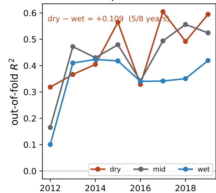
E. Richness prediction, climate
