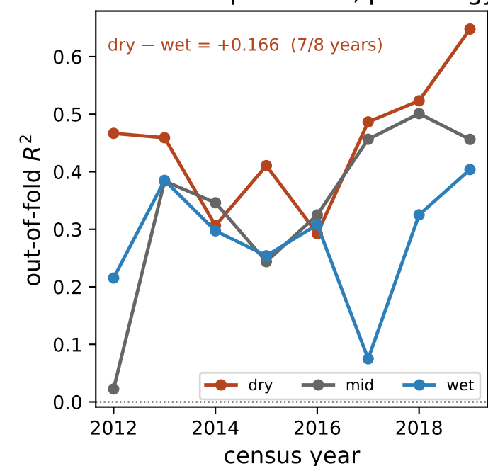
F. Richness prediction, phenology
