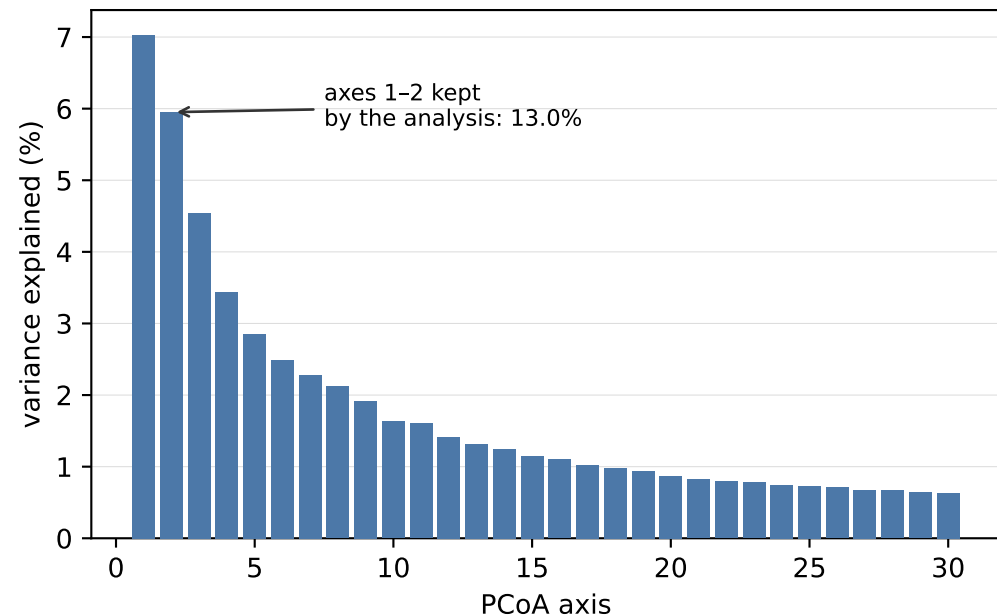
a No dominant axis, no elbow
