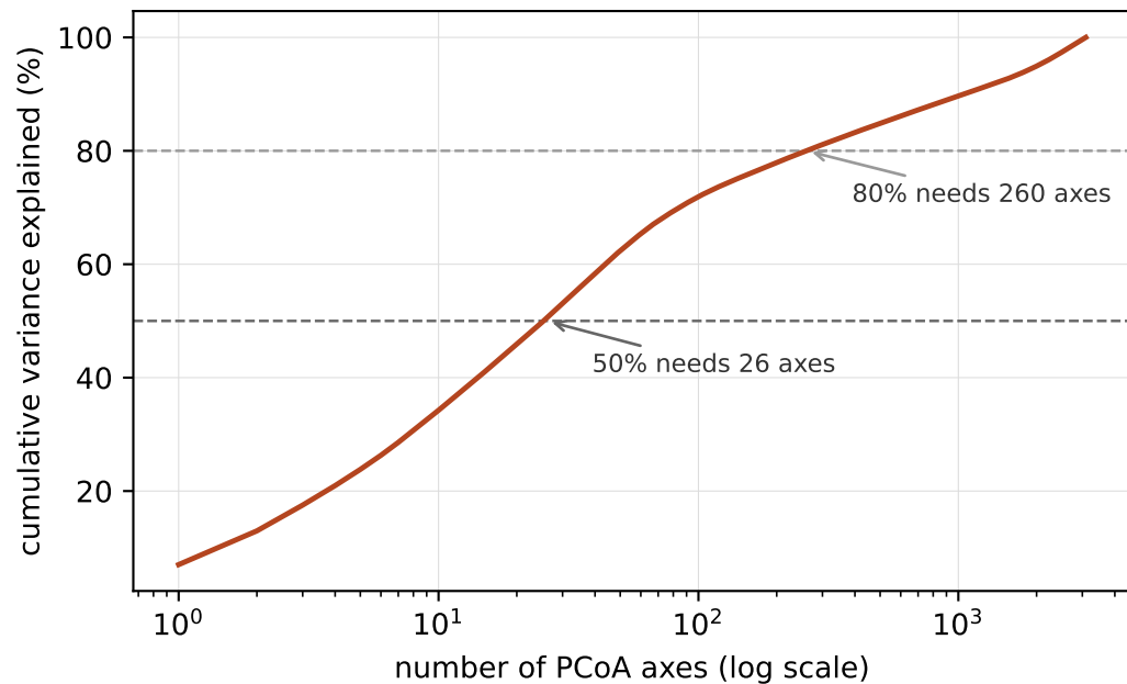
b Half the floristic turnover needs 26 axes
