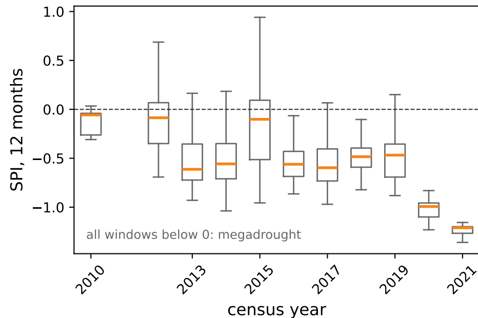
A. Water stress over the census window
