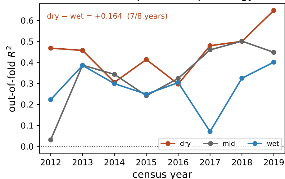
D. Richness prediction, phenology
