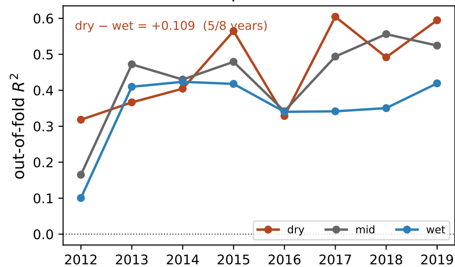
C. Richness prediction, climate
