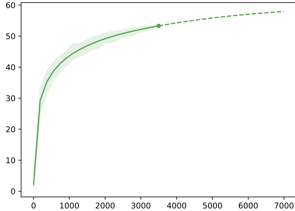
Phylogenetic Hill diversity (meanPD)
