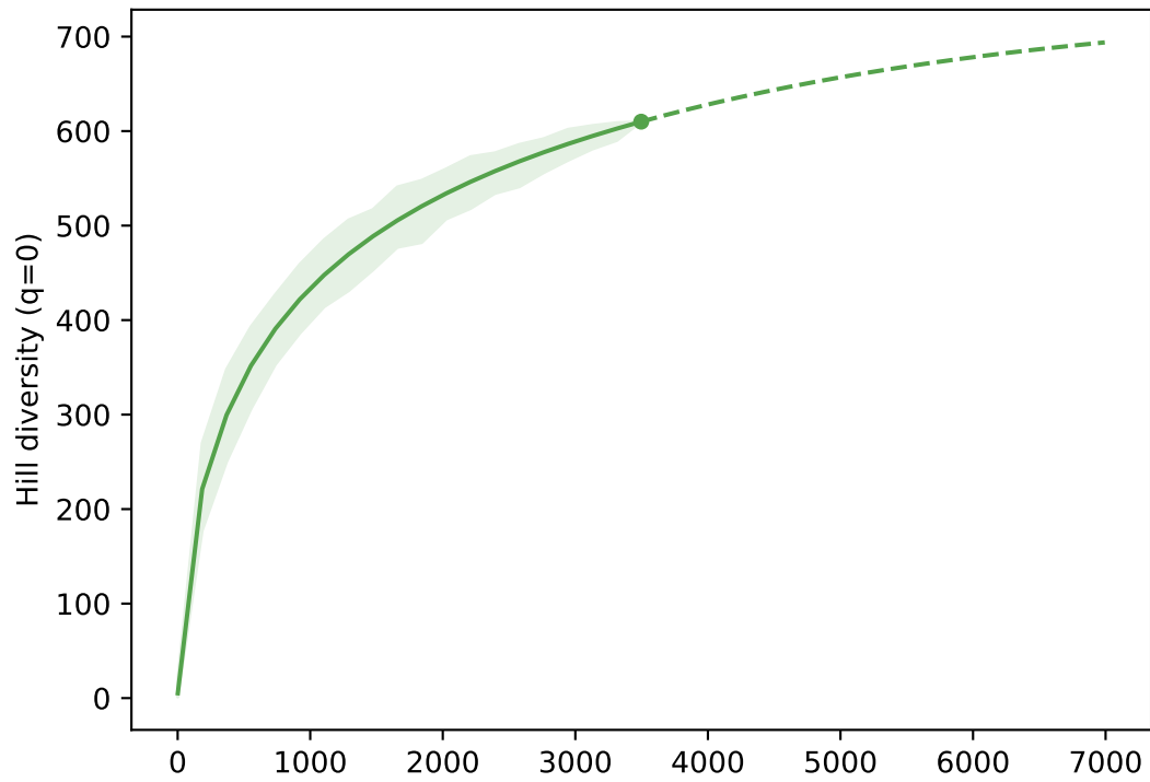
Taxonomic Hill diversity
