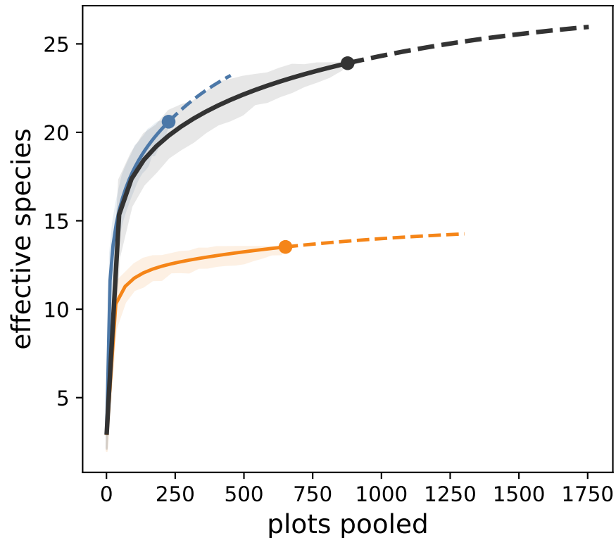
Phylogenetic diversity (PD), q = 0
