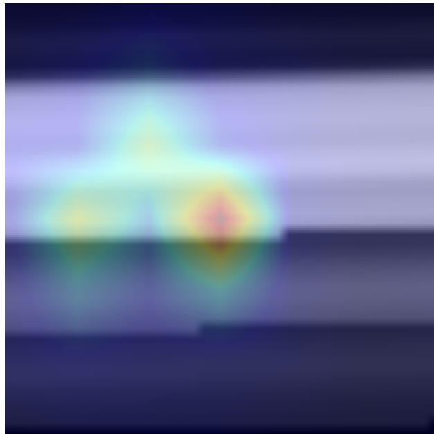
LAI: Grad-CAM on 2D image (embedding)
