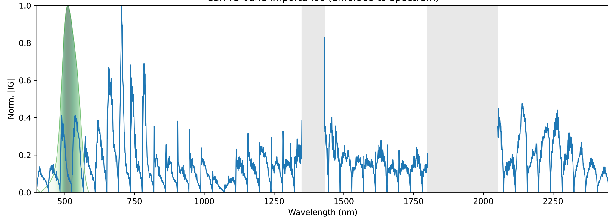
Car: IG band importance (unfolded to spectrum)
